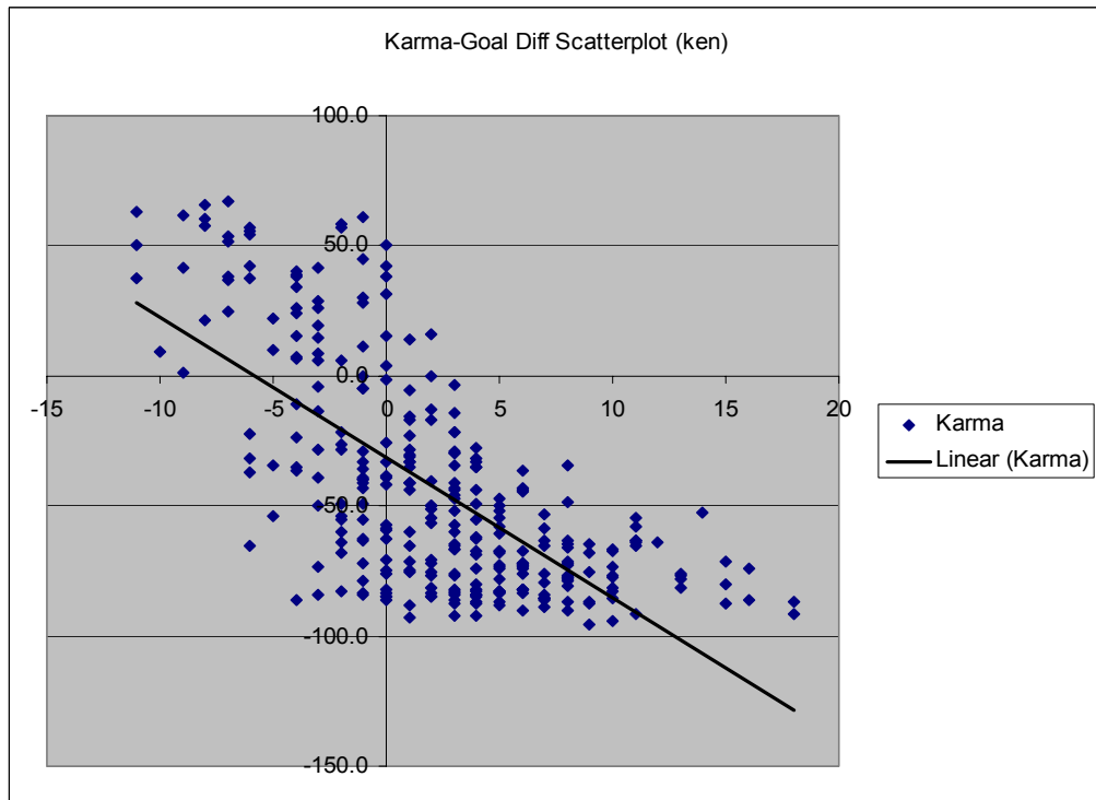
Figure 6.2: Scatter plots of karma and goal differential for ken
